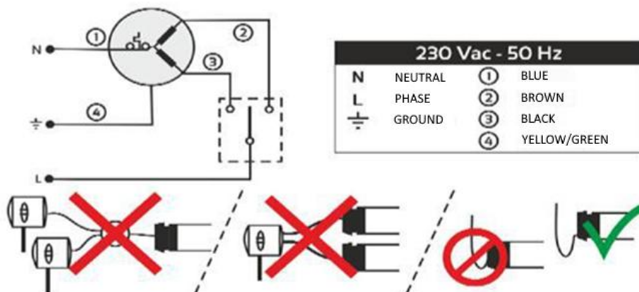
Fig. 3 Electric drive with switch
