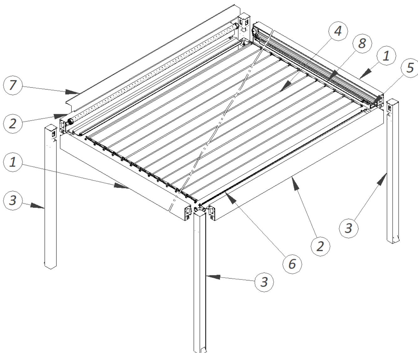
Fig.1 Tarasola Technic View - Graphic representation
